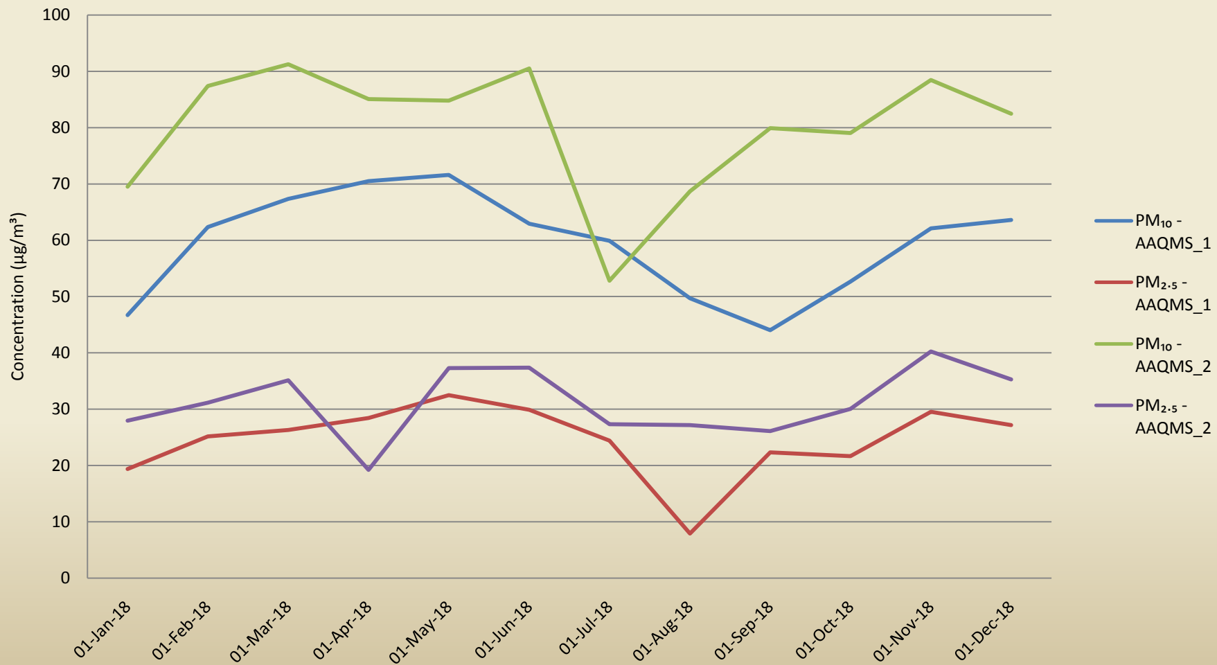
Annual Ambient Trend of Particulate Matter in M/s. Sanjay Gandhi Thermal Power Station, Dist. Umaria (M.P.)
