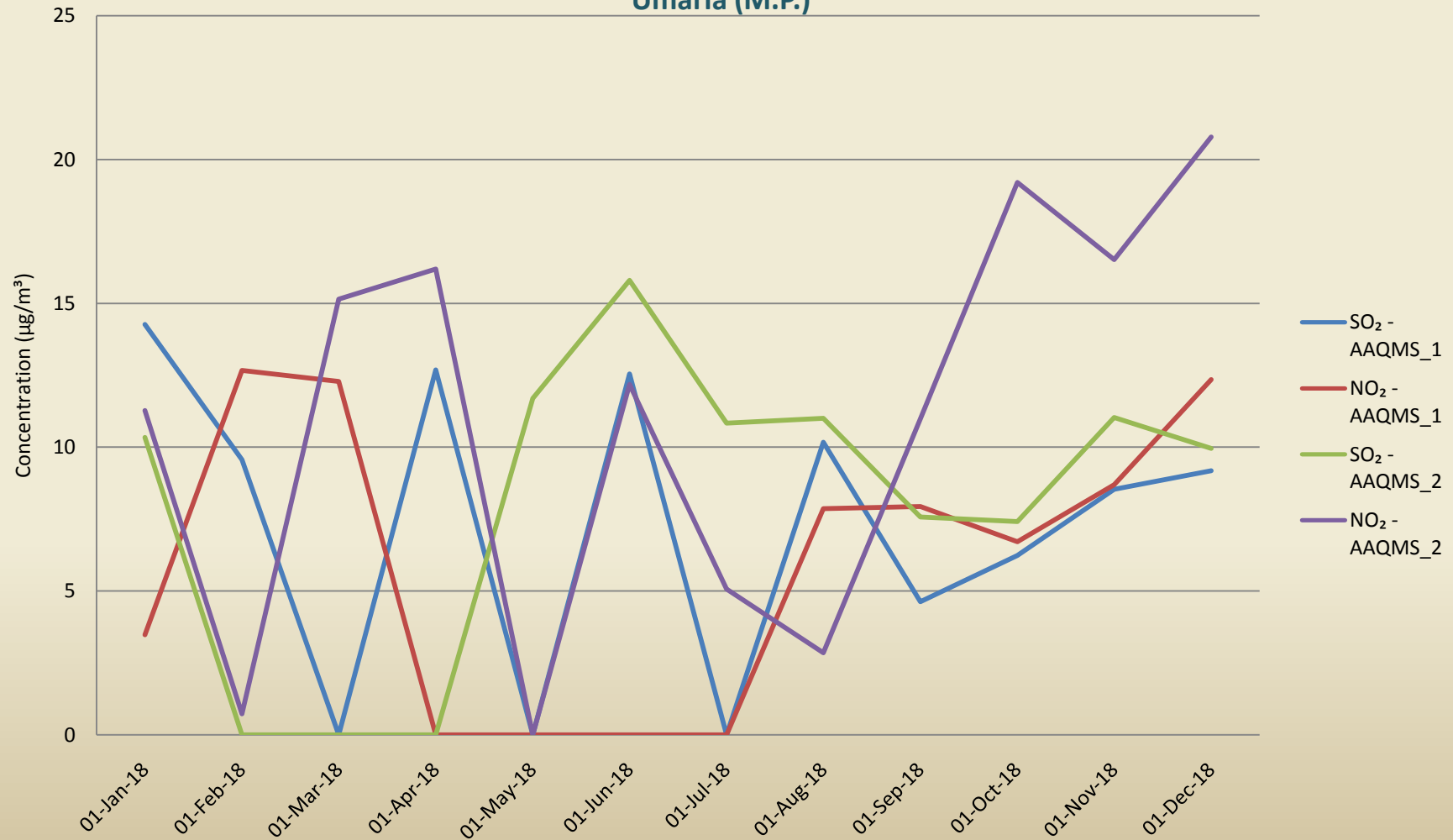
Annual Ambient Trend of Gaseous in M/s. Sanjay Gandhi Thermal Power Station, Dist. Umaria (M.P.)
